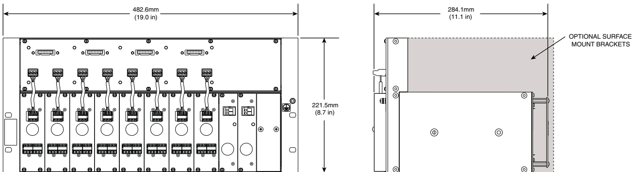
Figure 4. ROUTE-MASTER RM100 Fieldbus Power-Supply/Conditioner with Connector Panel. (RM110 Power Tray Combined with RM100 has same dimensions).
