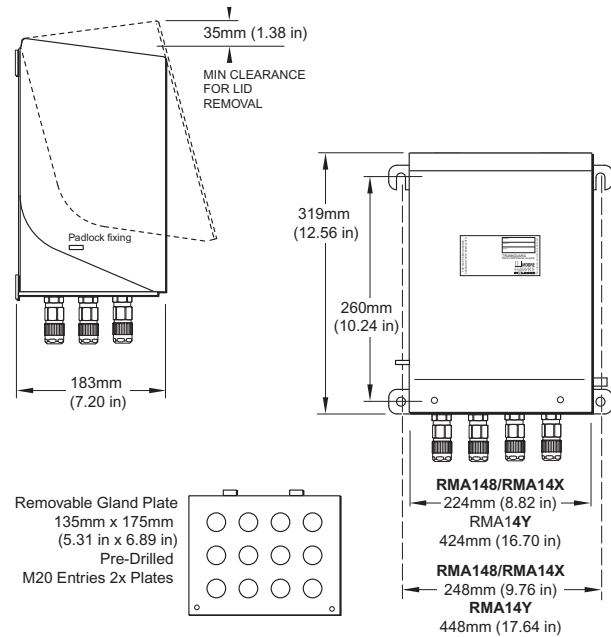
Figure 9. Stainless Steel 316 with E-Z Vertically Removable Lid and Bottom Entry Cable Gland Plate Installation Dimensions for 8-Spur (RMA148), 10-Spur (RMA14X) and 20-Spur (RMA14Y) Device Couplers.
