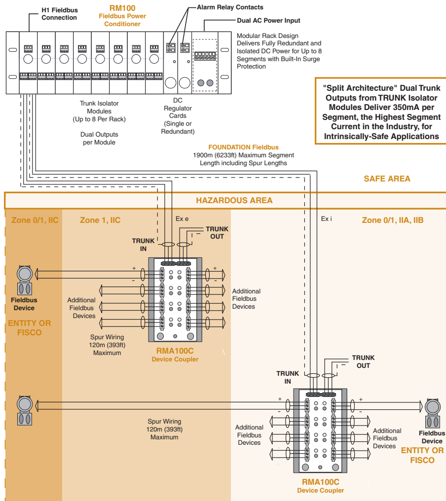
Figure 2A. The ATEX approved, FISCO compatible ROUTE-MASTER features Device Couplers that mount directly in IIC areas (Model RMA100C) and delivers 350mA per segment into hazardous locations.
