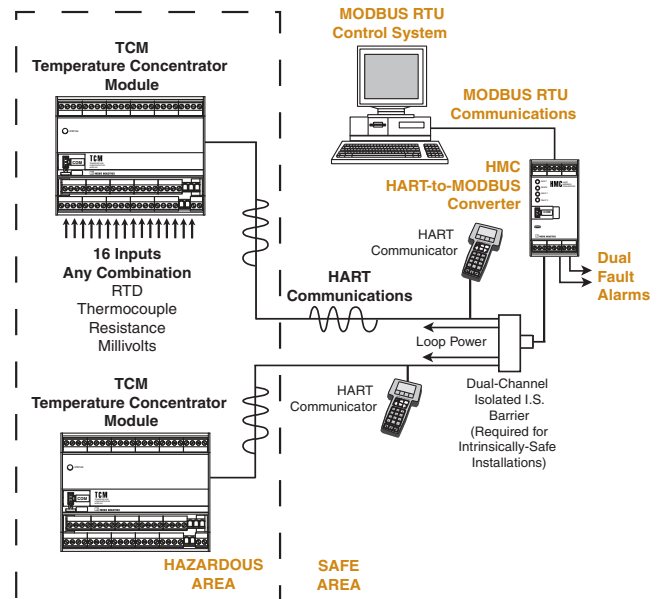
Figure 5. TCS in Intrinsically-Safe* MODBUS RTU Communications Mode.
